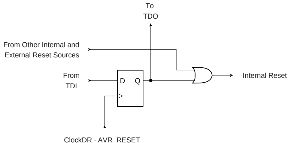
Figure 86. Reset Register
